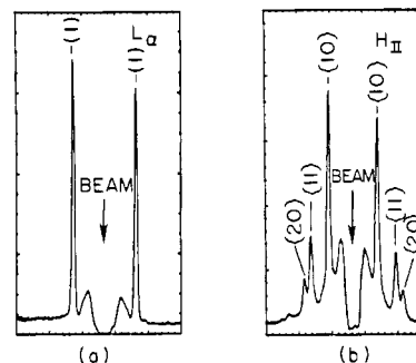
FIGURE 1: Azimuthal integrations of the two-dimensional X-ray diffraction patterns of aqueous DOPE (a) at 2 ^{\circ}\text{C} , when the system is in the L_{\alpha} phase, and (b) at 15 ^{\circ}\text{C} , when the system is in the H_{II} phase. The arrow indicates the position of the unscattered X-ray beam, blocked by a beam stop. The first-order L_{\alpha} peak indicated by the vertical lines in (a) is at (52.0\text{ \AA})^{-1} . In (b) lines indicate peaks whose positions index to an H_{II} lattice with first-order peak at (66.2\text{ \AA})^{-1} . The left-right asymmetry in peak intensity arises from the fact that no detector flat-field correction was applied to the data.
